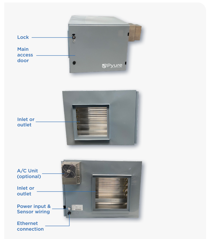
Figure 6: MVP16™ unit components
