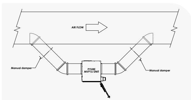
Figure 10: MVP16™ Duct bypass
