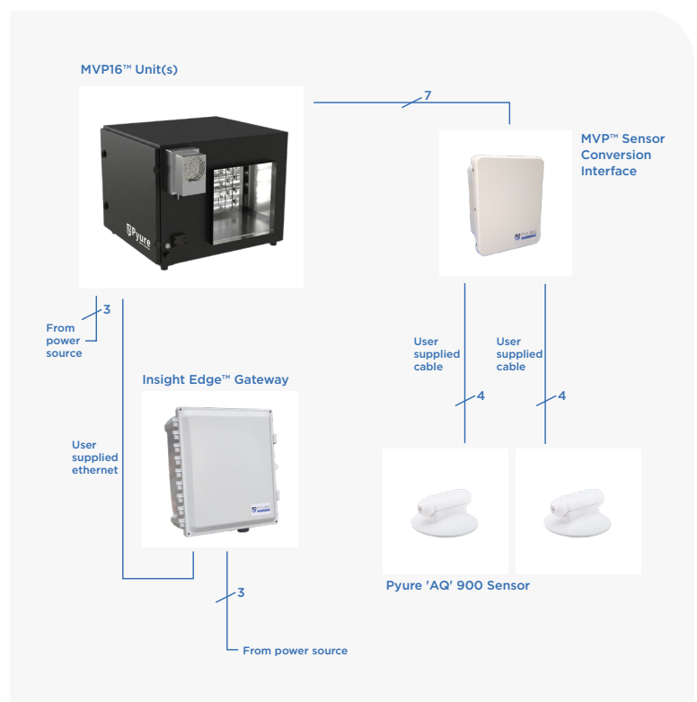
Figure 5: MVP16 System sample configuration with two Pyure 'AQ' 900 Sensors
